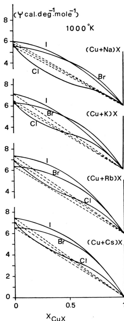
Fig. 3. \psi vs composition for the systems (Cu, Me)X.
